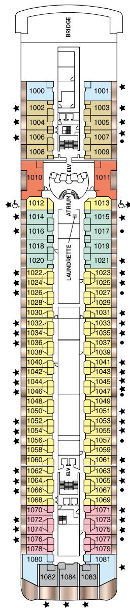
DECK 10
