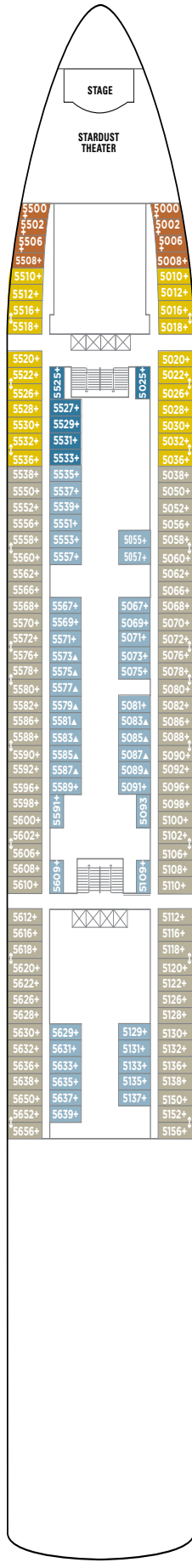
DECK 5
